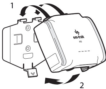
Figure 12 AIS transceiver mounting
