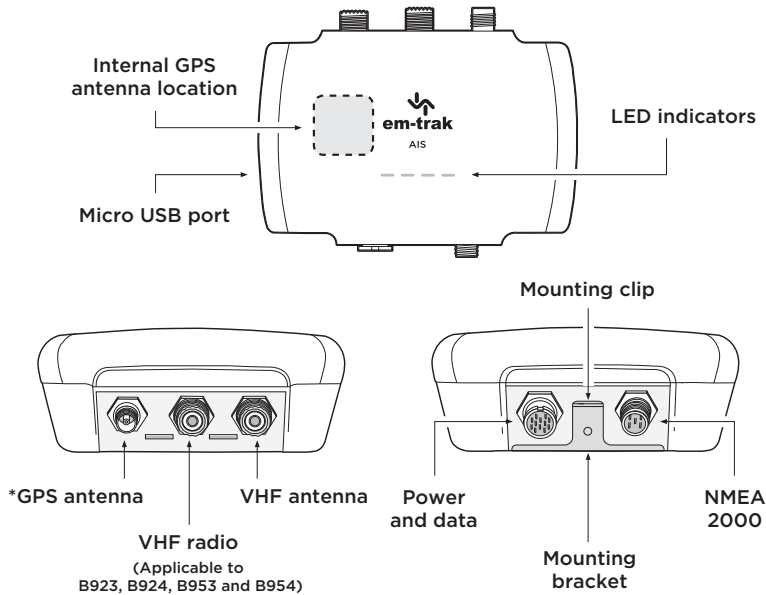
Figure 1 AIS transceiver overview
