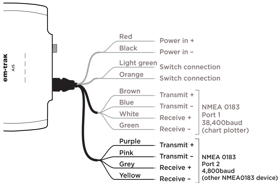
Figure 18 Connecting to your NMEA 0183 sensor
