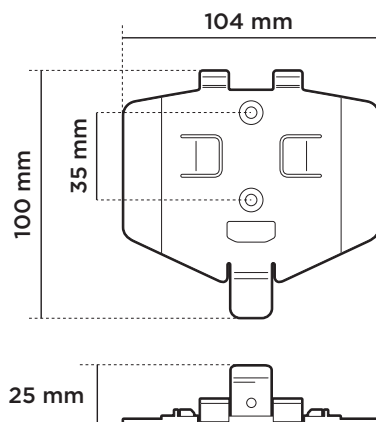
Figure 10 AIS transceiver dimensions
