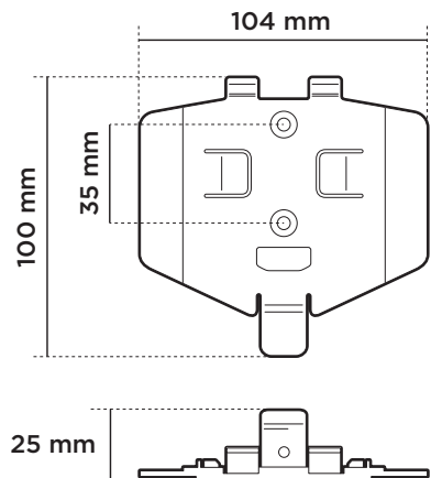
Figure 2 Transceiver dimensions
