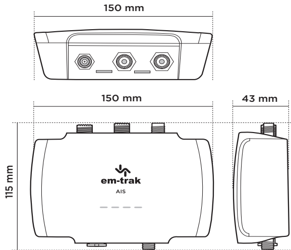
Figure 2 Transceiver dimensions
