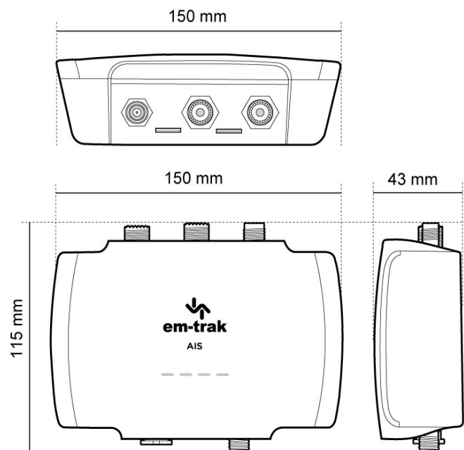
Figure 11 : Transceiver dimensions
