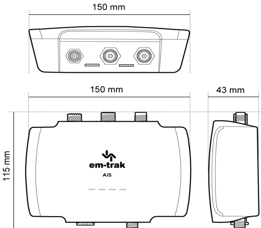
Figure 3 : Transceiver dimensions
