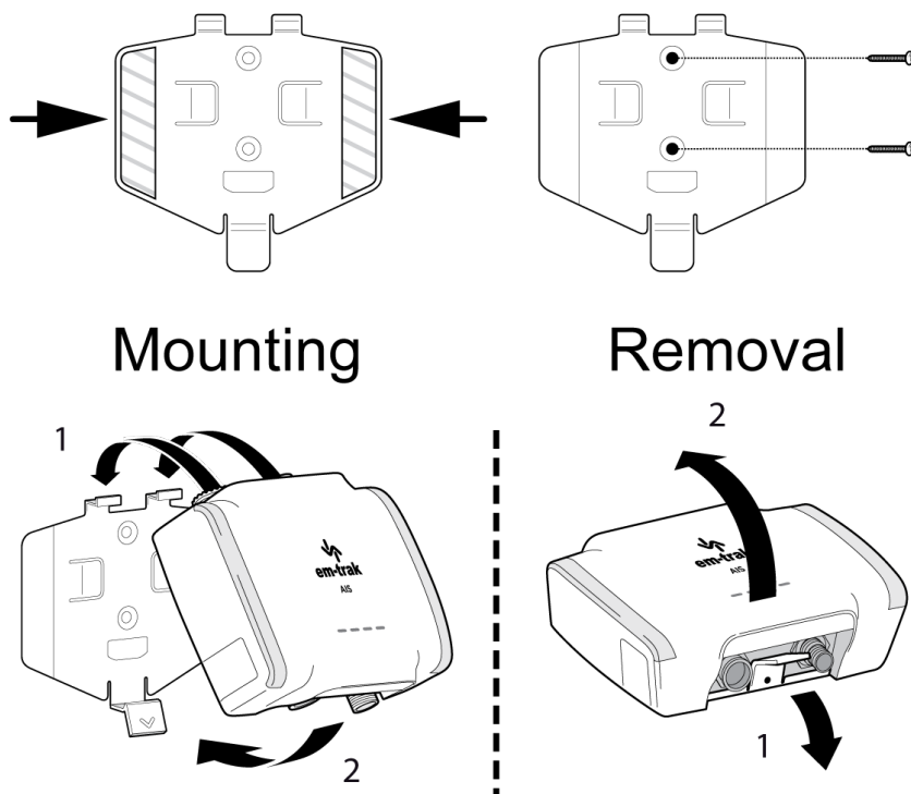
Figure 13 : AIS transceiver mounting
