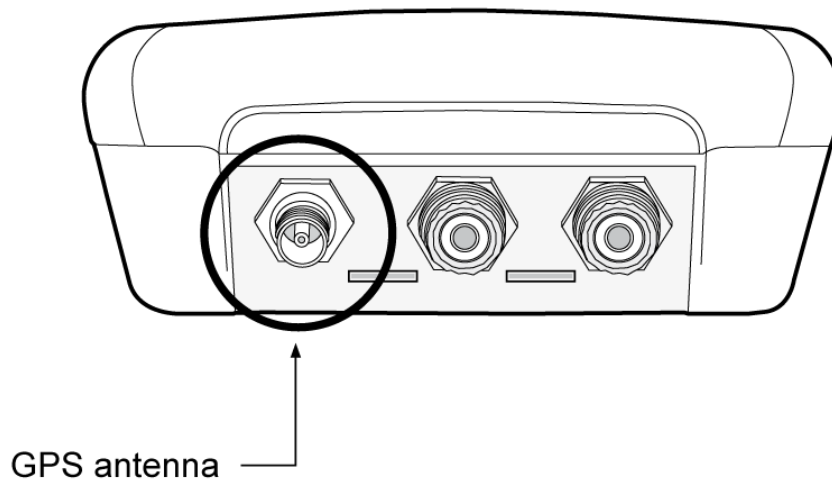
Figure 8 : GPS antenna connector
