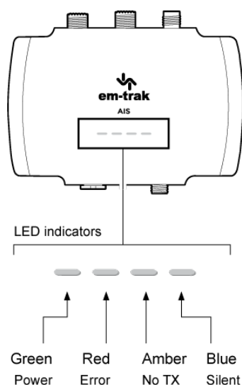
Figure 21 : LED indicator location on the AIS transceiver unit
