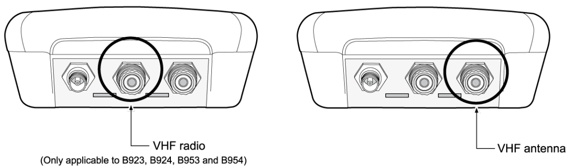
Figure 7 : VHF antenna connector
