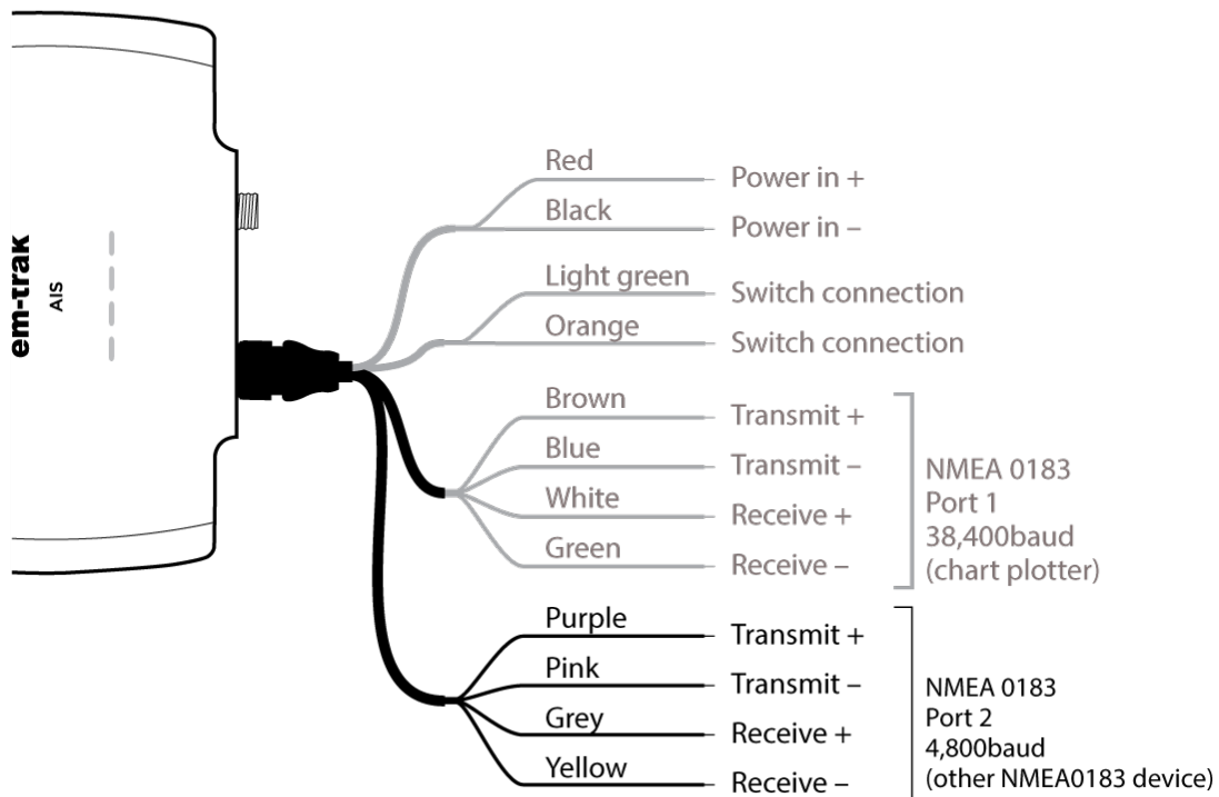
Figure 19 : Connecting to your NMEA 0183 sensor
