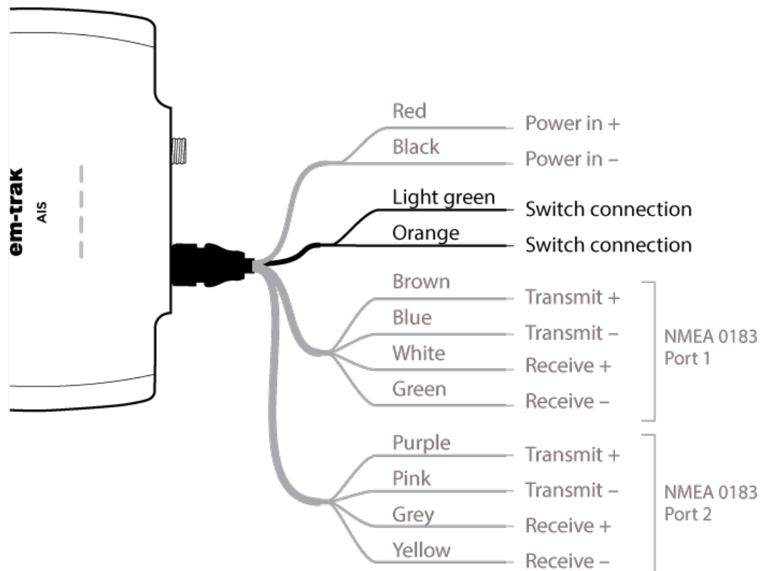
Figure 22 : Connecting an external switch
